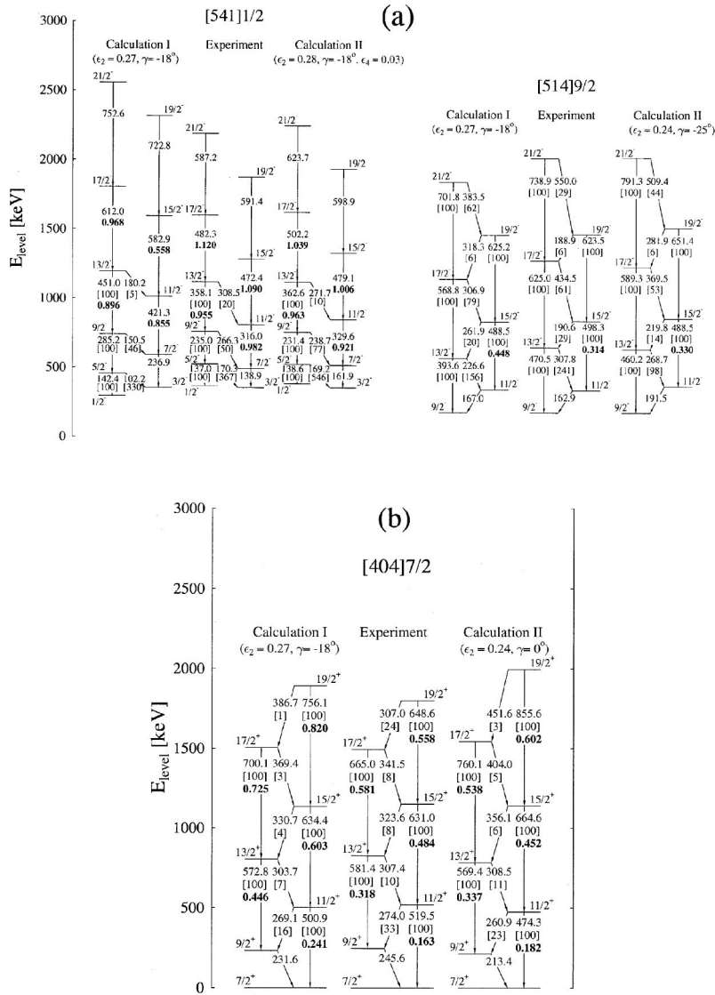
FIG. 4. (a) Low-lying negative-parity bands in ^{133}\text{Nd} compared to calculations I and II. The calculated band-head energies are set equal to the experimental ones. See also text. (b) The same as in (a), but for the [404]7/2 band.
